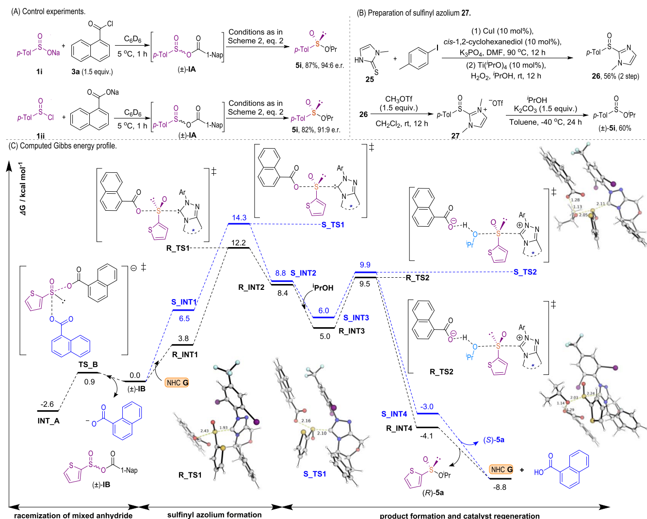
Scheme 5. (A) Control Experiments, (B) Preparation of Sulfinyl Azolium, and (C) Computed Gibbs Energy Profile; INT_A Is the Complex Formed between Mixed Anhydride IB and 1-Naphthoate; See Figures S16 and S19 for All DFT-optimized Structures
