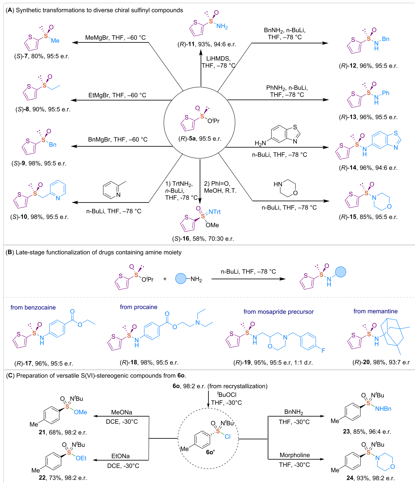
Scheme 4. Synthetic Transformations of the Catalytically Obtained Chiral Sulfinate Esters and Sulfinamides
