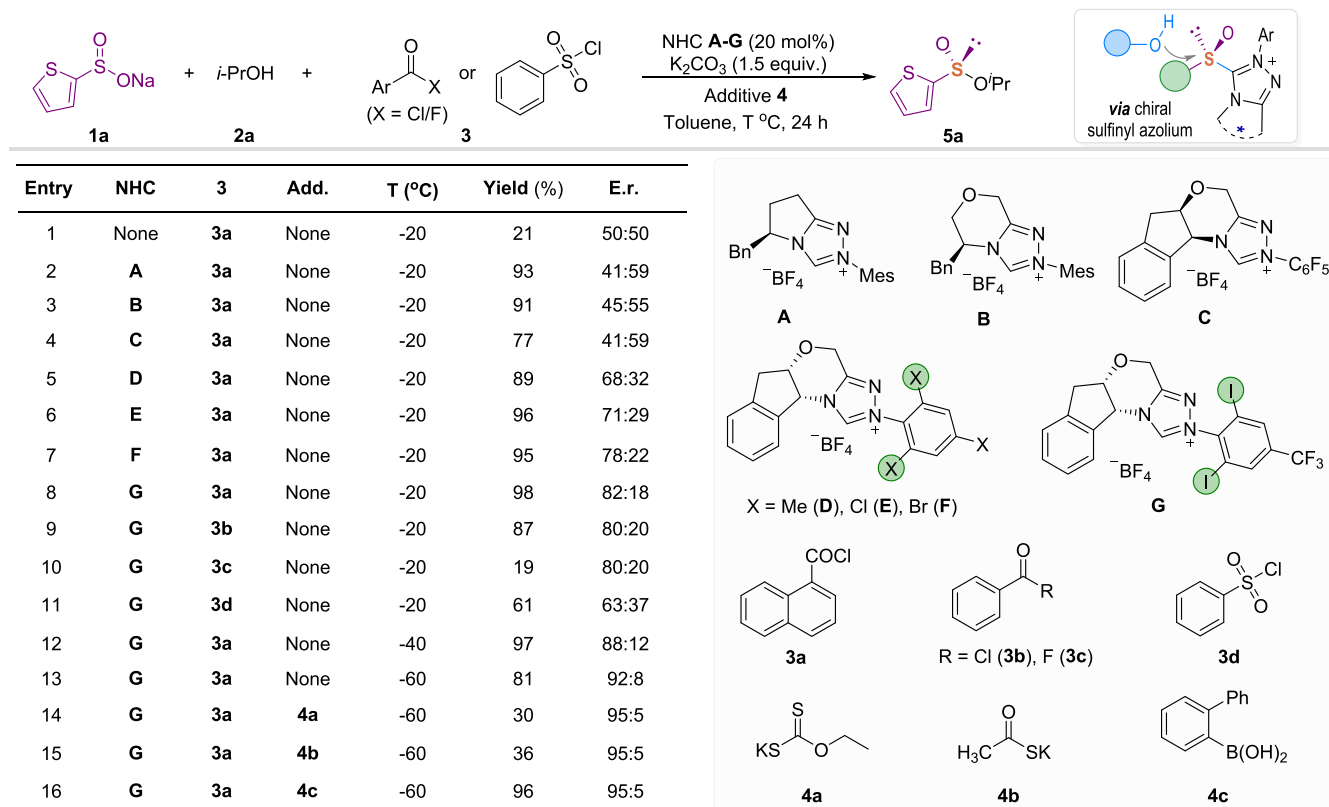
Scheme 1. Optimization of the Carbene-catalyzed Enantioselective Condensation of Sulfinate 1a and Alcohol 2a a
