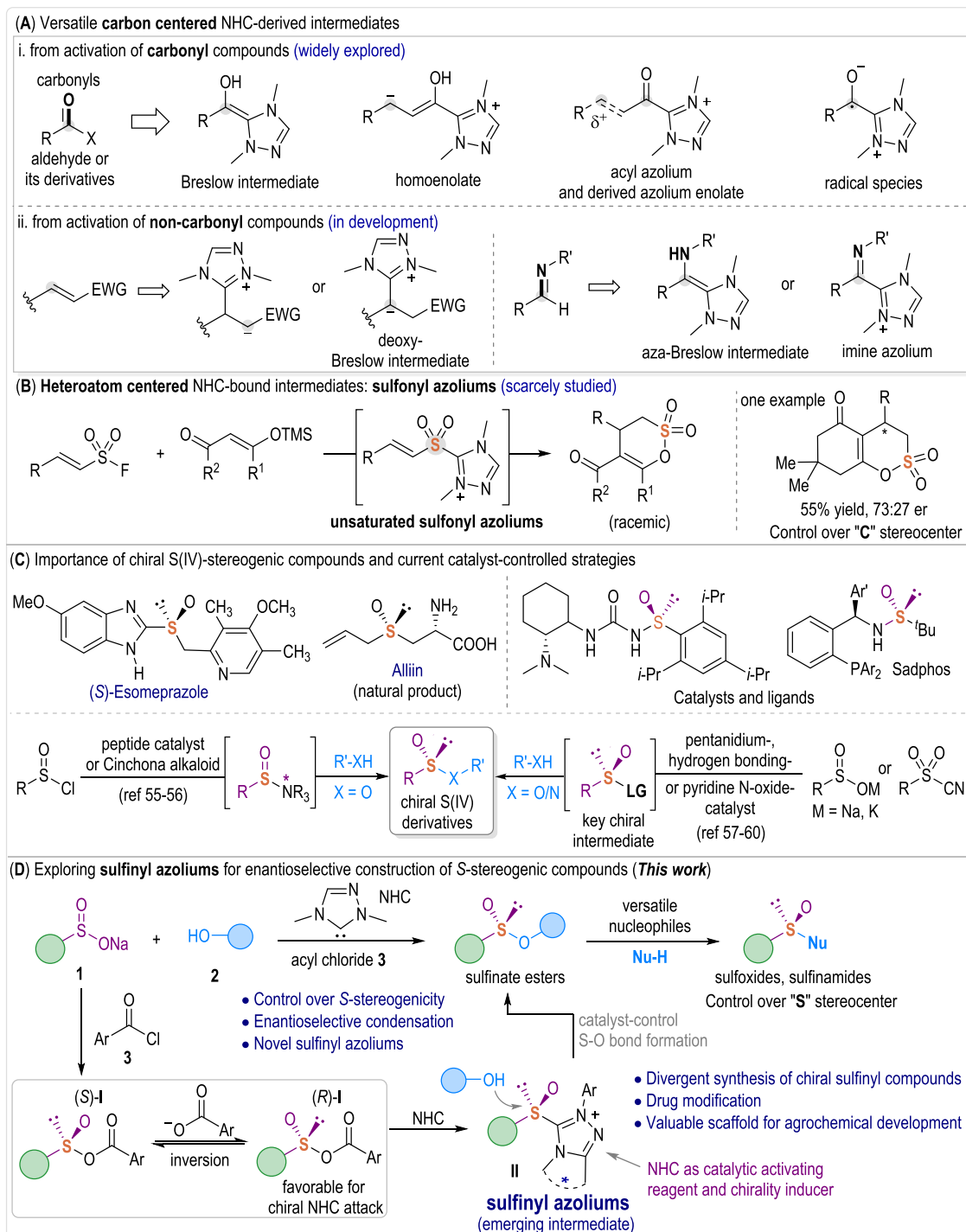
Figure 1. (A) Representative carbon-centered NHC-bound reactive intermediates. (B) Pioneering study on the carbene-derived sulfonyl azolium intermediate. (C) Importance of S-chiral compounds and current catalytic synthetic approaches. (D) Our proposed approach for preparation of various S-stereogenic compounds enabled by unprecedented sulfinyl azoliums by carbene activation of mixed sulfinic anhydrides.
